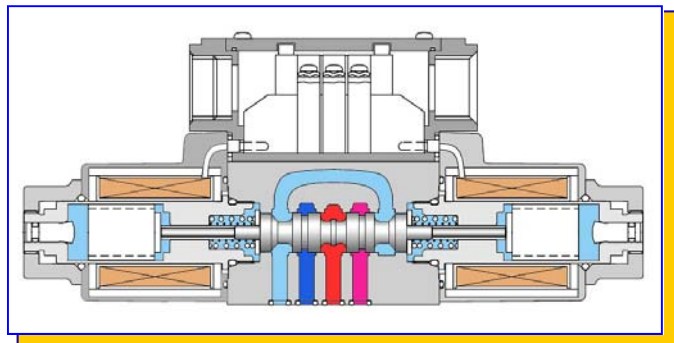
1/8" (CETOP3) Sub-Plate Mounting (F)-(S)-DSG-01-**-**-70 / 7090
